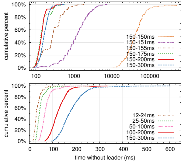
Figure 12: The time to detect and replace a crashed leader. The top graph varies the amount of randomness in election timeouts, and the bottom graph scales the minimum election timeout. Each line represents 1000 trials (except for 100 trials for “150-150ms”) and corresponds to a particular choice of election timeouts; for example, “150-155ms” means that election timeouts were chosen randomly and uniformly between 150ms and 155ms. The measurements were taken on a cluster of 5 servers with a broadcast time of roughly 15ms (results for a cluster of 9 servers are similar).
